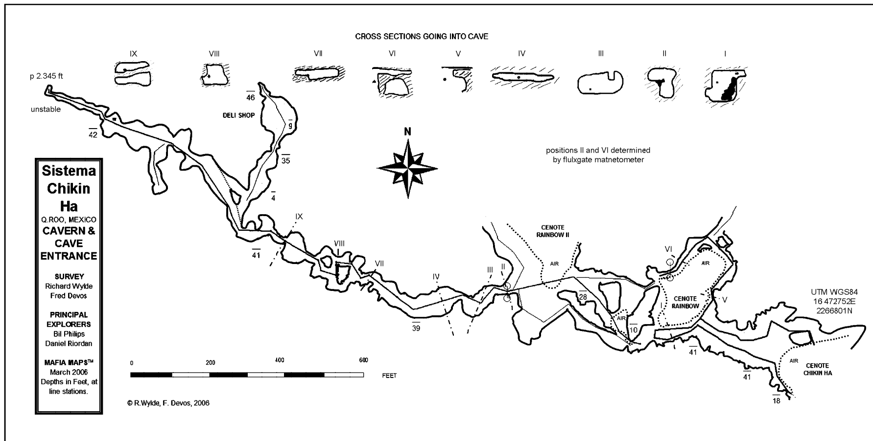
Sistema Chikin Ha (part) Puerto Aventuras Quintana Roo AMCS Activities Newsletter 30, p. 152, 2007
